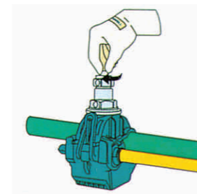
Turn the nut by hand, and fix the connector in suitable location.
