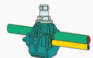
Insert the main wire, if there are two layers of insulated lay in the main cable, should strip a certain length of the first in length of the fist insulated lay from inserted end.
